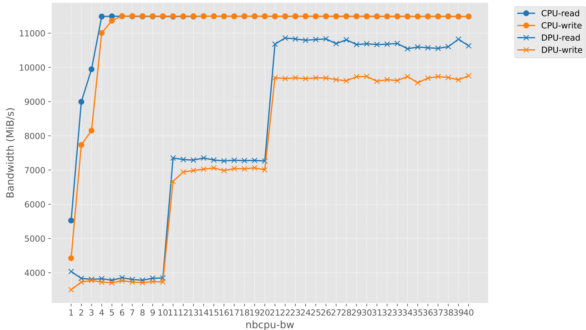
Bandwidth vs nbcpu-bw (CPU vs DPU)
